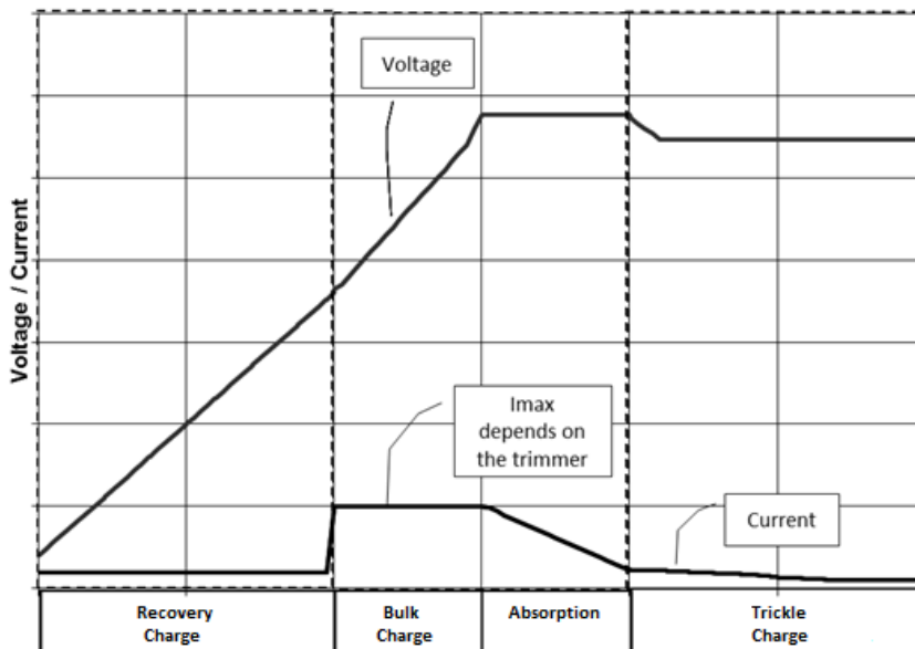
CB1224xA - CB1224xAJ Charging Diagram
