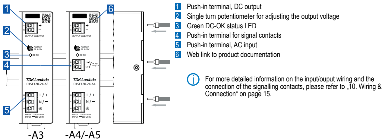
Fig. 1: Description of user elements
