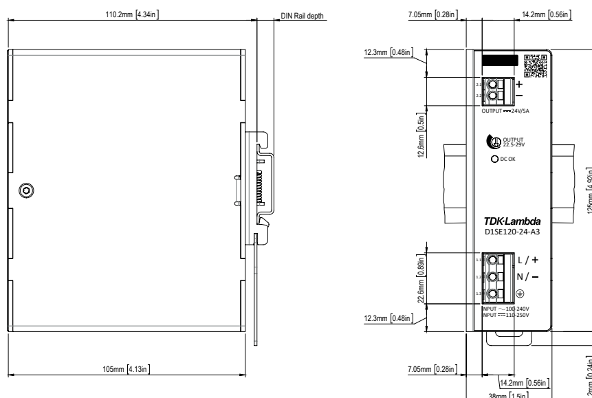
Fig. 16: Dimension drawing of D1SE120-24-A3
