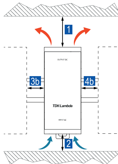
Fig. 19: Installation clearances to passive components
