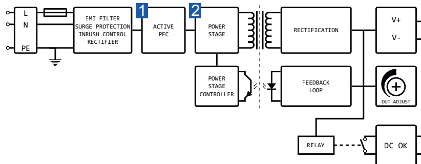
Fig. 24: Block diagram of -A4/-A5 models
