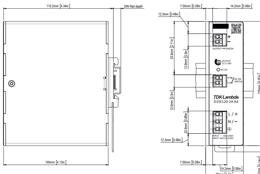
Fig. 17: Dimension drawing of D1SE120-24-A4/A5
