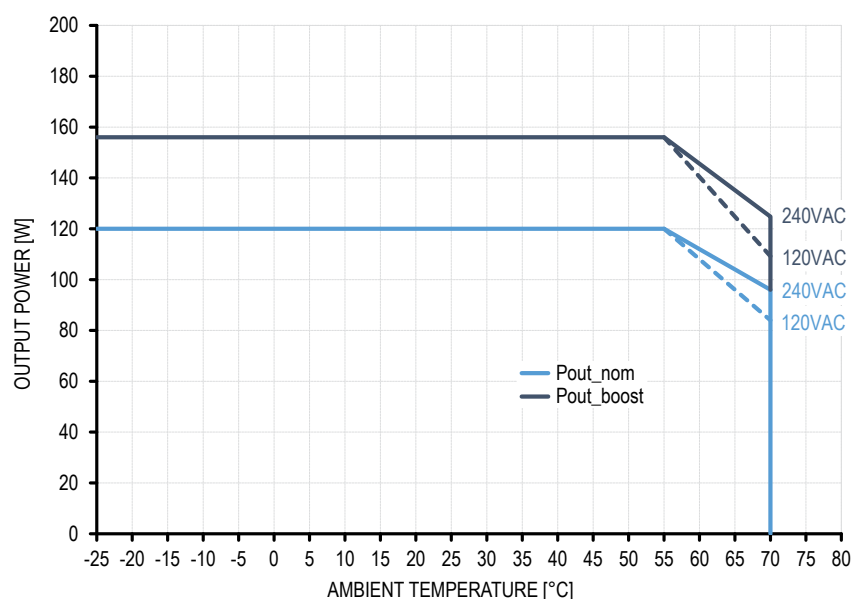
Fig. 14: Available output power in dependence of the ambient temperature for 90° rotated mounting position
