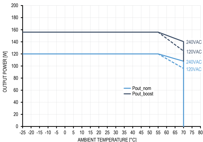
Fig. 13: Available output power in dependence of the ambient temperature for normal and 180° rotated mounting positions
