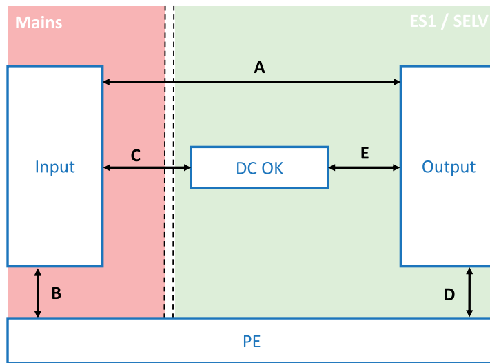
Fig. 25: Schematic of the insulation paths
