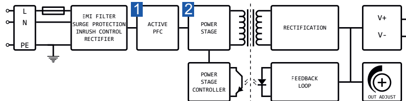
Fig. 23: Block diagram of -A3 models
