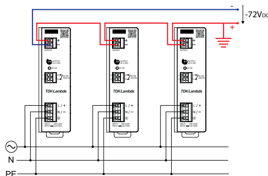
Fig. 29: Connection scheme for series operation with negative voltage level
