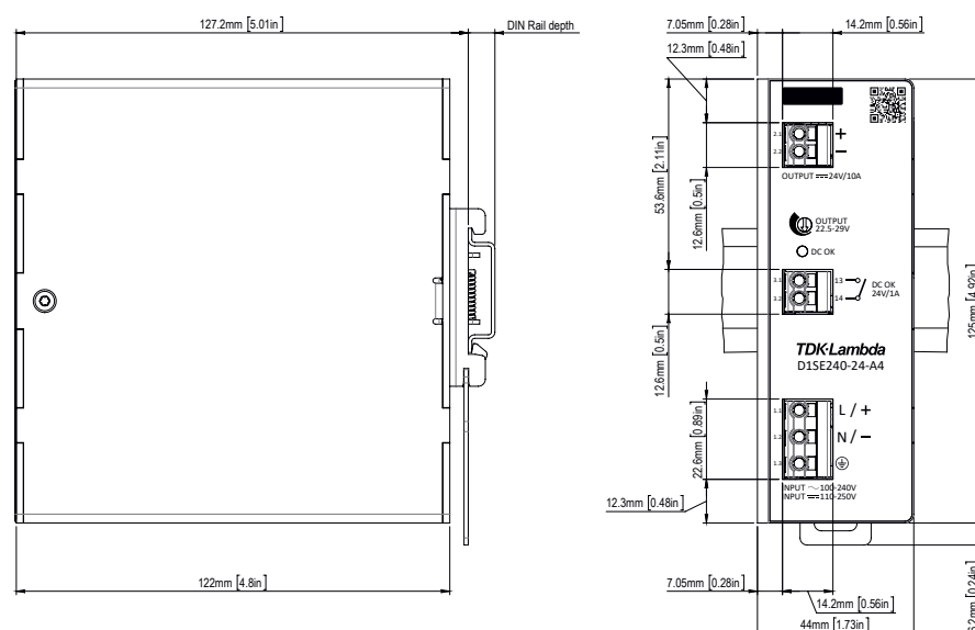
Fig. 17: Dimension drawing of D1SE240-24-A4/A5
