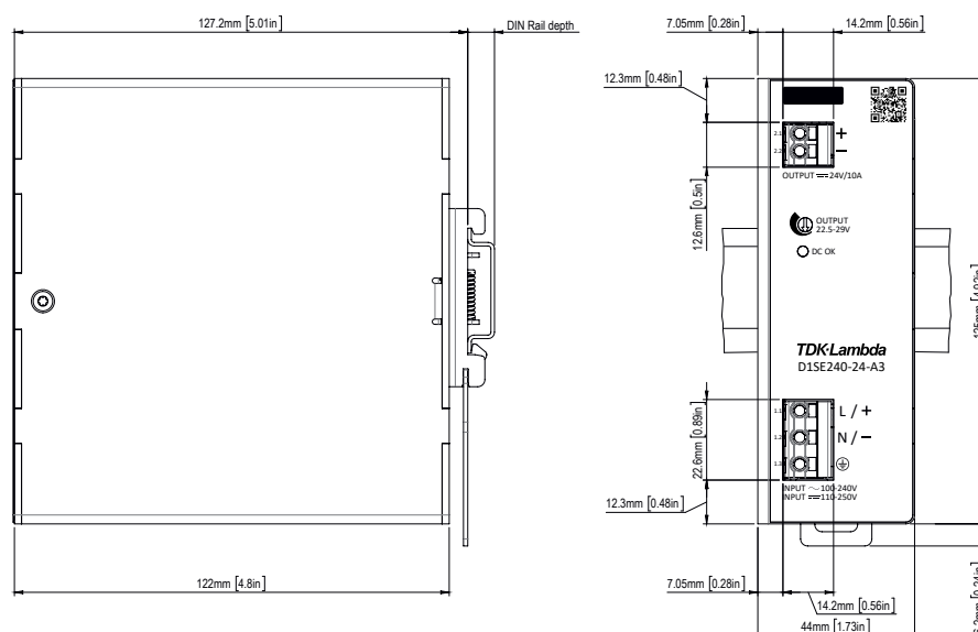
Fig. 16: Dimension drawing of D1SE240-24-A3
