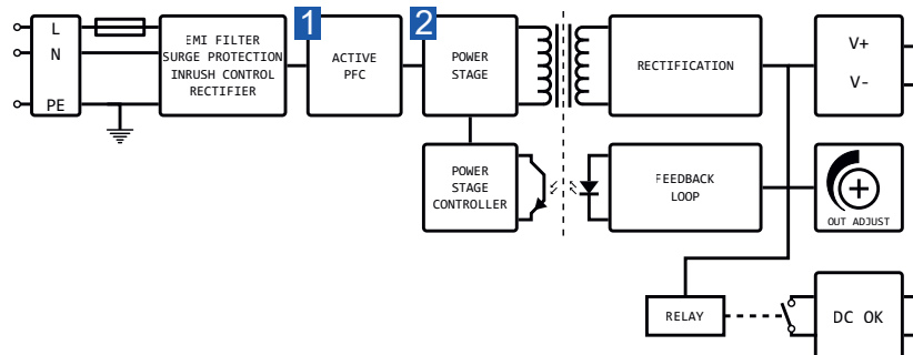
Fig. 25: Block diagram of -A4/-A5 models
