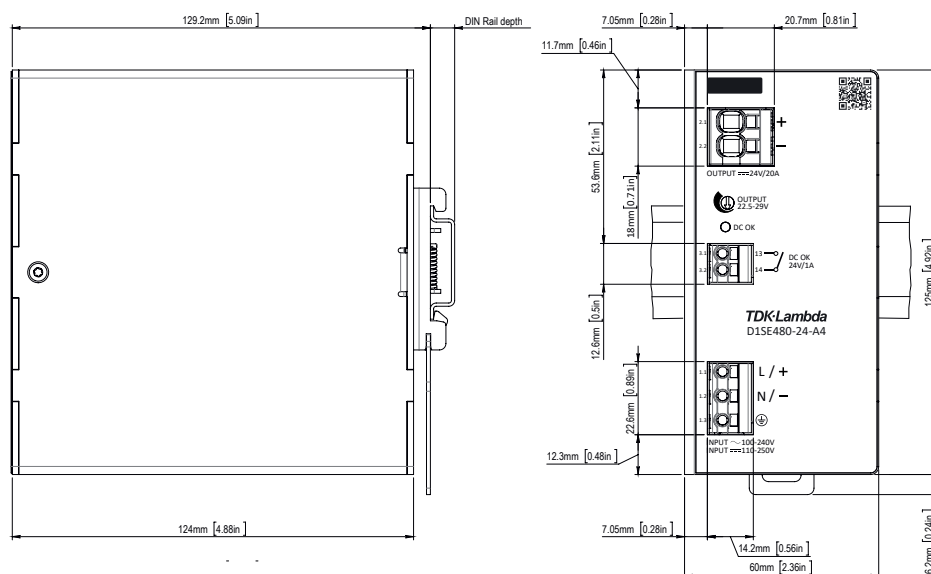
Fig. 18: Dimension drawing of D1SE480-24-A4/A5
