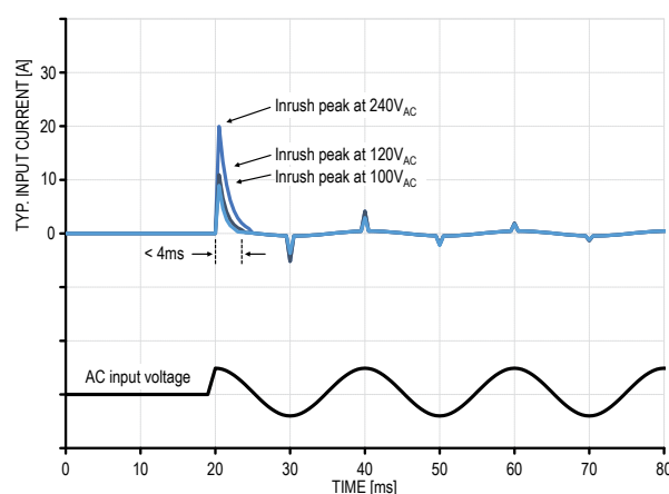
Fig. 6: Inrush current and energy during start-up phase
