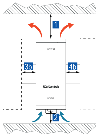
Fig. 20: Installation clearances to passive components
