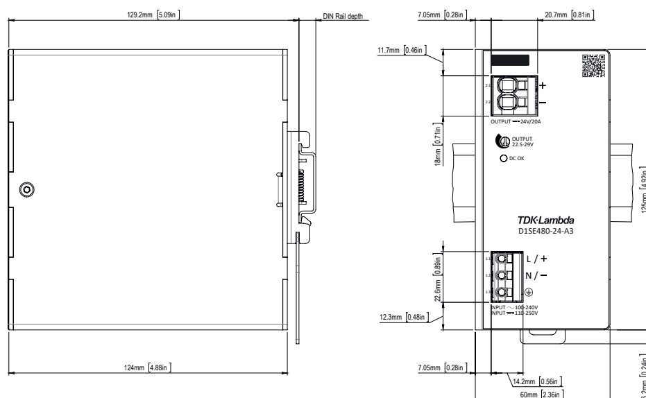
Fig. 17: Dimension drawing of D1SE480-24-A3
