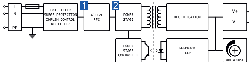
Fig. 24: Block diagram of -A3 models
