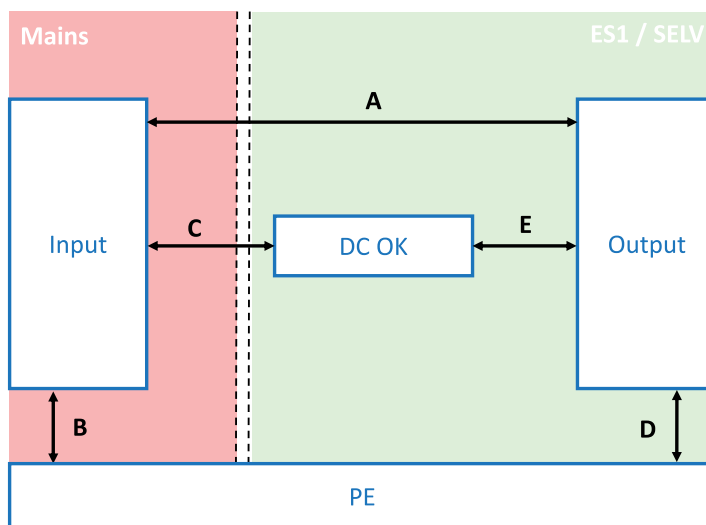
Fig. 26: Schematic of the insulation paths
