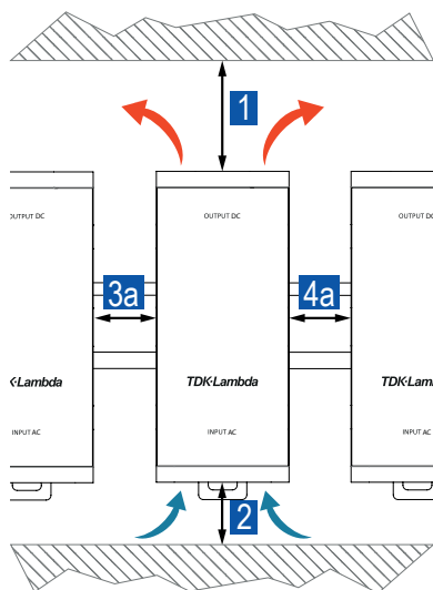
Fig. 19: Installation clearances to heat sources
