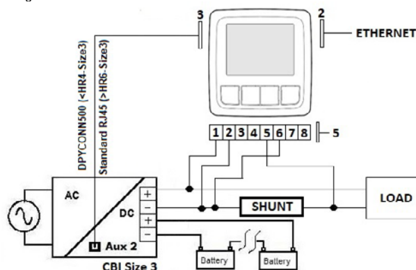
Fig. 4 – External Shunt connection for CBI Size 3
