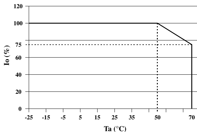
Output derating : Ta-Io
