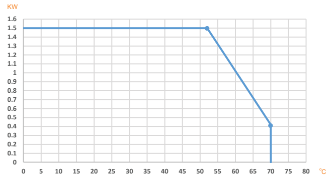
Fig. 2: Output Power vs. Temperature (C)
