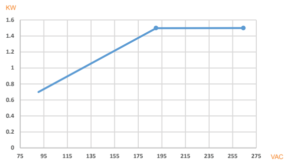
Fig. 3: Output Power vs. AC Input Voltage
