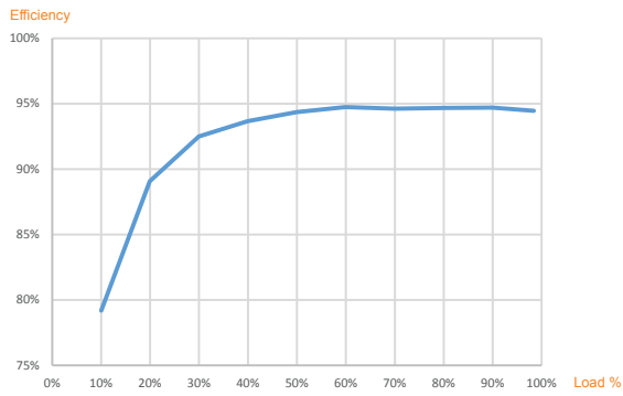
Fig. 1: 48VDC Power Module Efficiency
